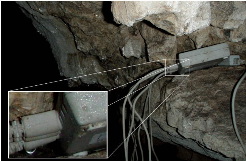
Fig. 9: Condensation droplets in CSB passage. Moisture on the logger (inset) demonstrates that the droplets formed during the study period.
